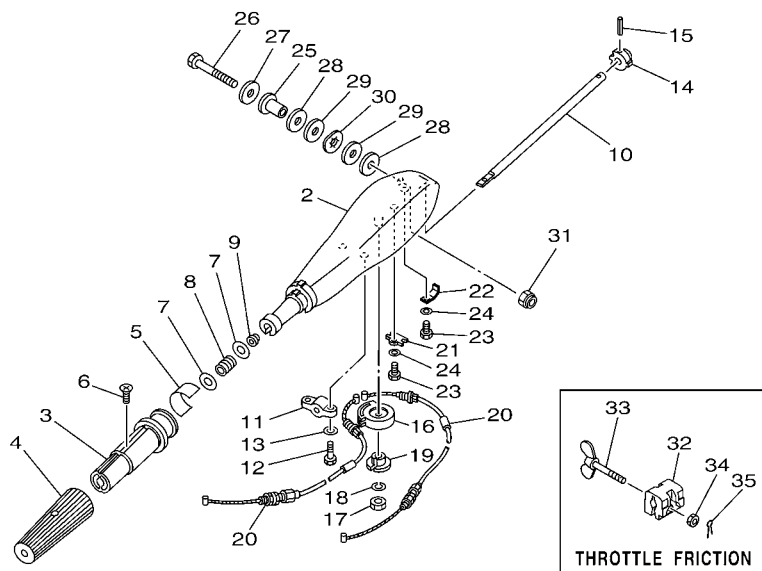
1 HANDLE STEERING ASSY Fig. 15, STEERING Ref. No. 2 to 35
