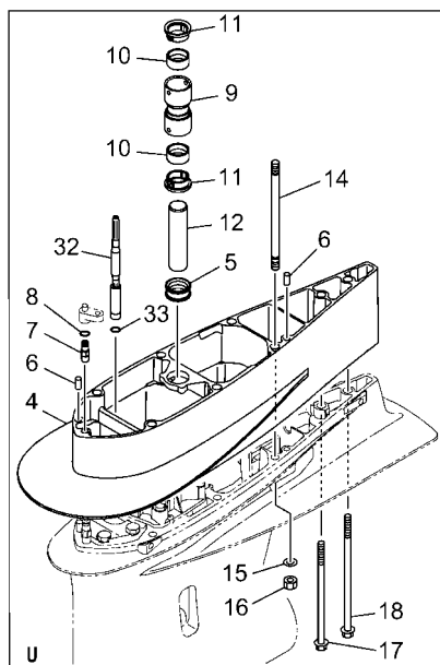
COUNTER ROTATION
