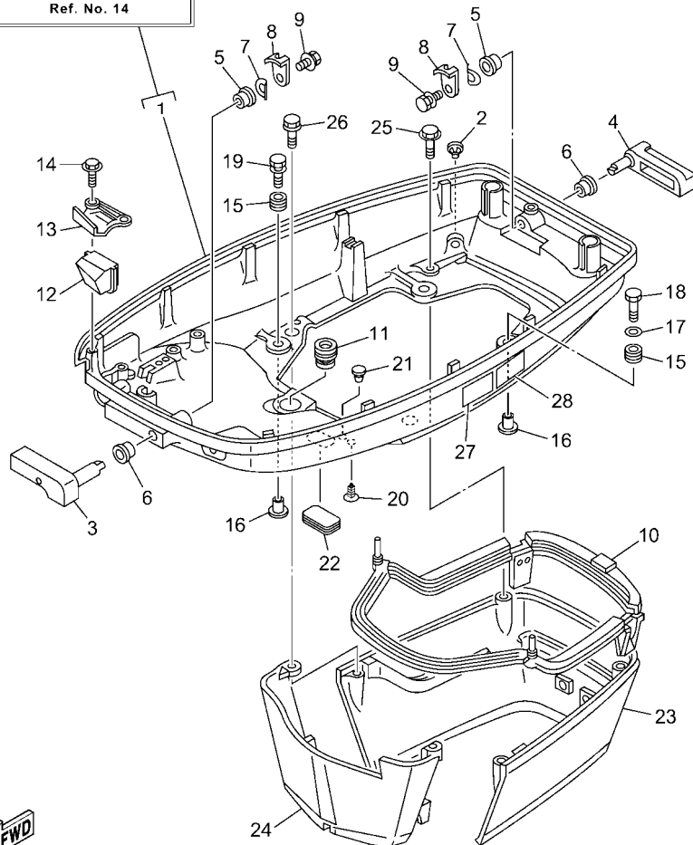
Fig. 14, BOTTOM COWLING Ref. No. 14
